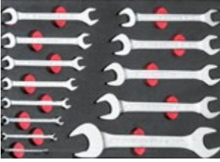
Grand Master Çekmece 2 - Sol Grand Master Series Drawer 2 - Left Kod / Code: 13000 005591 Sayfa / Page: 7
